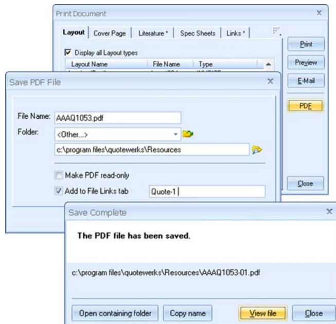
Figure 2: PDF Assembler
