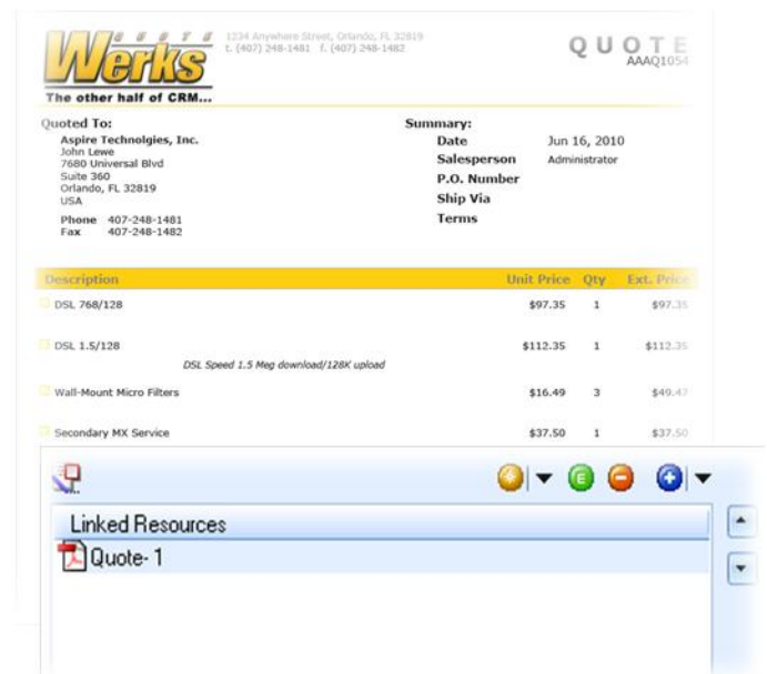
Figure 3: PDF Outputs
